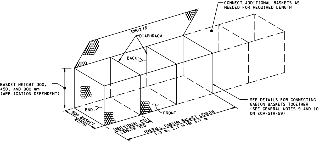
ISOMETRIC - TYPICAL GABION N.T.S.
