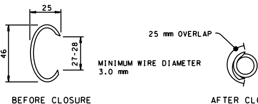
TYPE 2 FASTENER OVERLAPPING RING
