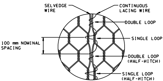
WOVEN MESH GABION LACING DETAIL TYPE 3 FASTENER LACING WIRE
