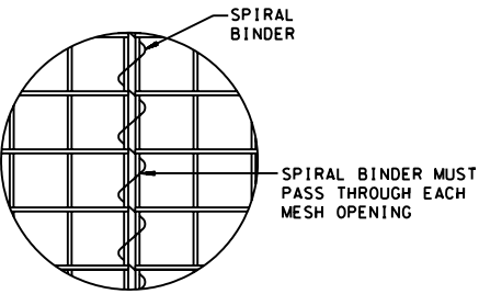
WELDED MESH GABION SPIRAL BINDER LACING DETAIL
