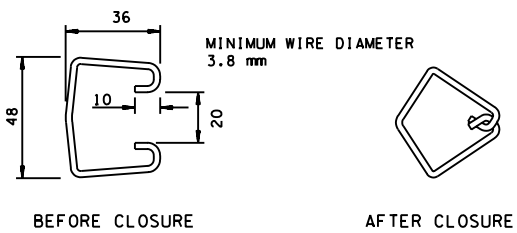
TYPE 1 FASTENER INTERLOCKING WIRE
