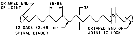
TYPE 4 FASTENER SPIRAL BINDER
